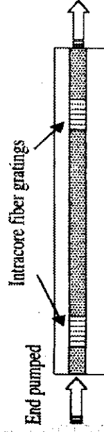
Fig. 1. Schematic representation of the investigated acoustic DFB-FL sensor.
