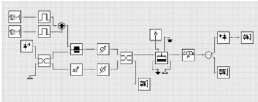
Fig. 3. Schematic model of the Q device simulated with the VPI_ComponentMaker™ software tool.
