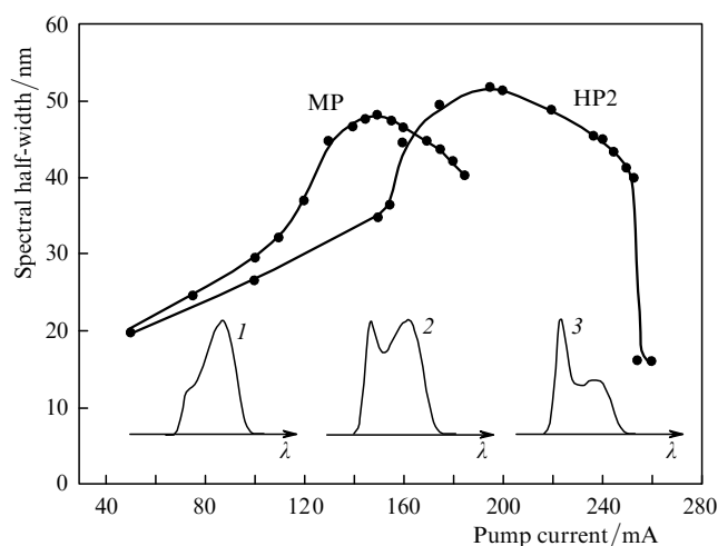
Figure 1. Typical dependences of the half bandwidth \Delta\lambda (FWHM) on the injection current I_{\text{SLD}} for SLD-37 modules of the MP category ( P_{\text{FS}} = 4 - 6 mW) and HP2 category ( P_{\text{FS}} = 20 - 30 mW). The insets show typical shapes of the spectrum for a low pump level (1), in the region of maximal \Delta\lambda (2) and for a high pump level (3).
