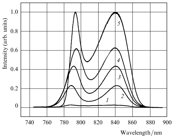
Figure 4. Spectra of the output emission of a two-section SLD for different combinations of injection currents: I_1 = 105 \text{ mA} , I_2 = 0 \text{ mA} (1), I_1 = 192 \text{ mA} , I_2 = 20 \text{ mA} (2), I_1 = 251 \text{ mA} , I_2 = 30 \text{ mA} (3), I_1 = 289 \text{ mA} , I_2 = 45 \text{ mA} (4), I_1 = I_2 = 196 \text{ mA} (5).
