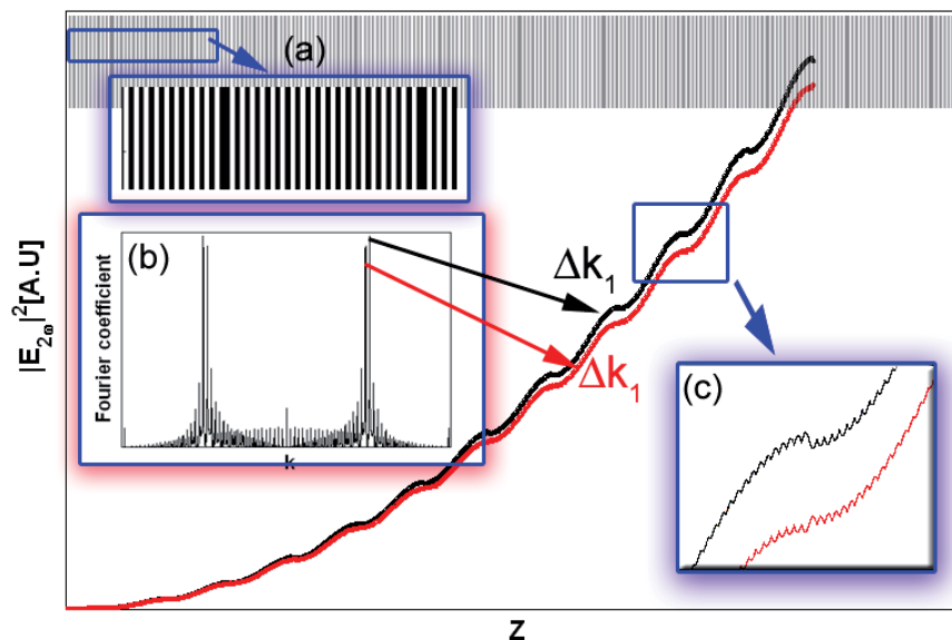
Figure 14 (online color at: www.lpr-journal.org ) Evolution of the square absolute of the generated waves in a quasiperiodic nonlinear photonic crystal. Inset (a) is the nonlinear pattern as a function of crystal position; inset (b) is the absolute value of the Fourier transform |G(\Delta k)| ; (c) is an expanded view of the square absolute of the two generated waves.
