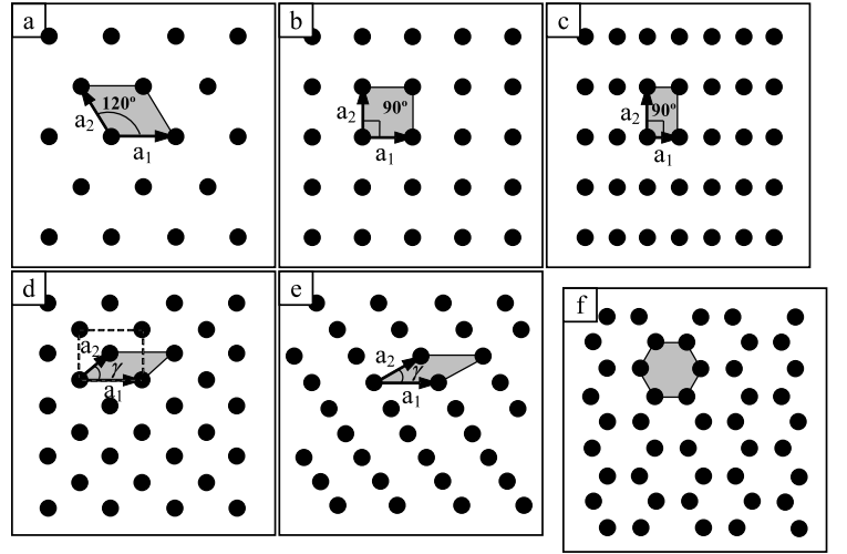
Figure 9 The six lattice types, five of them (a–e) are Bravais lattices: (a) hexagonal, (b) square, (c) rectangular, (d) centered-rectangular, where the dashed lines form a rectangle, (e) oblique. Panel (f) is a honeycomb lattice. The gray area in each one of the lattices refers to its unit cell.
