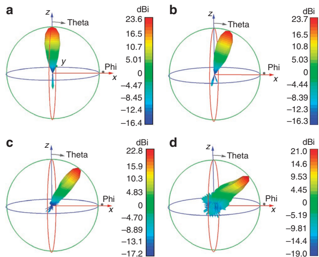
Figure 3 | Simulated 3D far-field radiation patterns of the 3D lens at 15 GHz. (a) The feeding source is located at the centre of the focal plane ( x=0 and y=0 ). (b–d) The feeding source is located 10, 20 and 30 mm off the centre of the focal plane ( x=-10, -20 and -30 \text{ mm} , and y=0 ).
