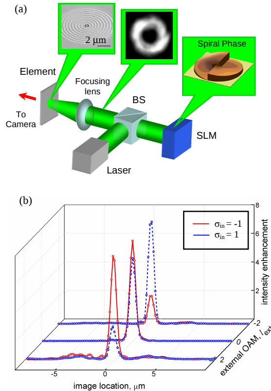
Fig. 4. Removal of the spin-degeneracy in circular corrugation by use of externally induced OAM. (a) experimental setup. A laser beam is modulated by a Spatial Light Modulator (SLM) to obtain a spiral phase and then incident through a Beam Splitter (BS) onto a coaxial aperture with circular corrugation. The transmitted light is captured in the image plane by the camera.
