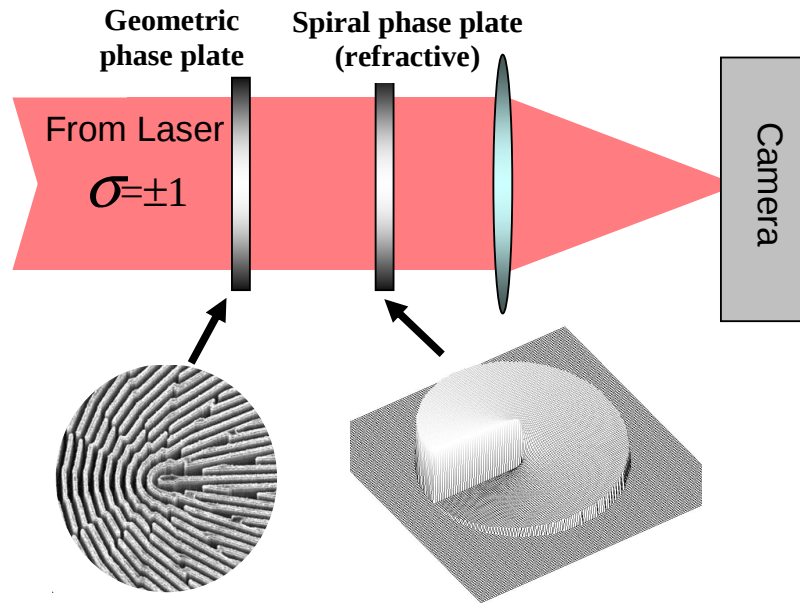
Fig. 1. Schematic illustration of the experiment.
