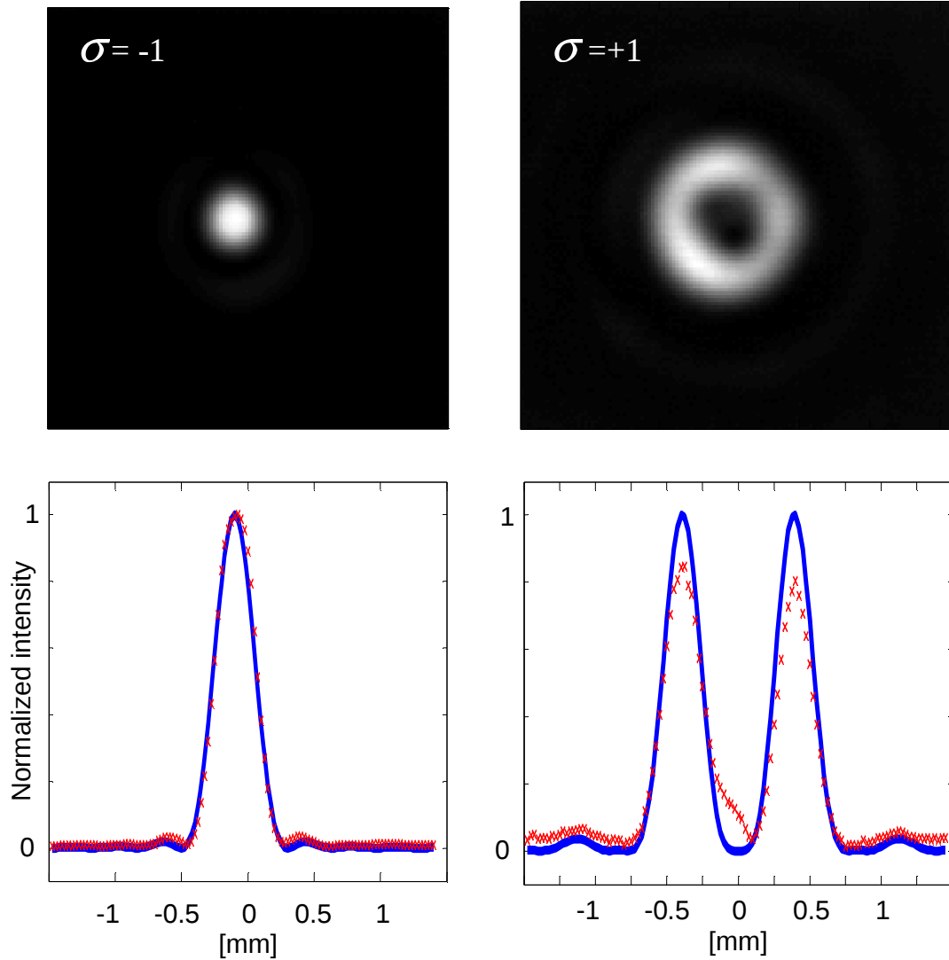
Fig. 2. Upper row shows the captured intensity distributions for different illumination helicities, (circular polarized light: left-handed \sigma = -1 , and right-handed \sigma = +1 ). The lower row shows experimental (red 'x's) and predicted (solid blue line) typical cross-sections.
