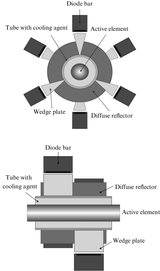
Figure 9. Scheme of a laser head with lens ducts used for coupling pump radiation [45, 46].
