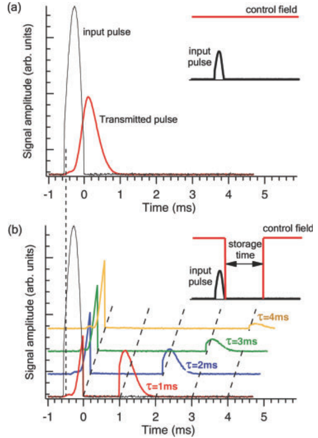
Figure 3 (online color at: www.lpr-journal.org ) Examples of measured signal field after propagation through a warm-Rb EIT medium with 22 torr Ne buffer gas: (a) slow light (constant control field); (b) stored light (flat control field during signal pulse writing and retrieval; zero control field during storage). In both cases the control field power was 900 \mu\text{W} . Insets show schematics of time-course for the control field and input signal pulse.
