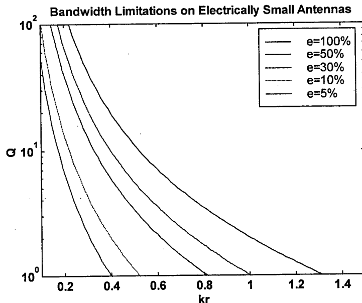
Figure 4-1 Theoretical calculation of omnidirectional antenna Q vs. r , the radius of an enclosing sphere, and the efficiency e emphasizes the limitations of small antennas for wide bandwidth operation.
