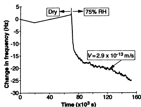
Fig. 4. Change in resonant frequency upon the addition of humid air; RH, relative humidity. The change in frequency represents immediate crack growth.
