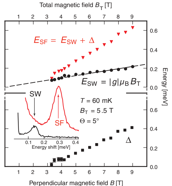
Fig. 4. Energies of the spin-wave mode (black circles) and the higher-energy spin-flip mode (red triangles). The black dashed line is a linear fit to the data using the standard Zeeman formula: E_{SW} = |g|\mu_B B_T . We find |g| = 0.42 , in agreement with the value expected for GaAs. Representative examples of the two spin excitation modes at two different laser energies (red line, 1522.6 meV; black line, 1522.4 meV) are shown in the inset. The black squares label the splitting \Delta between the two spin modes.
