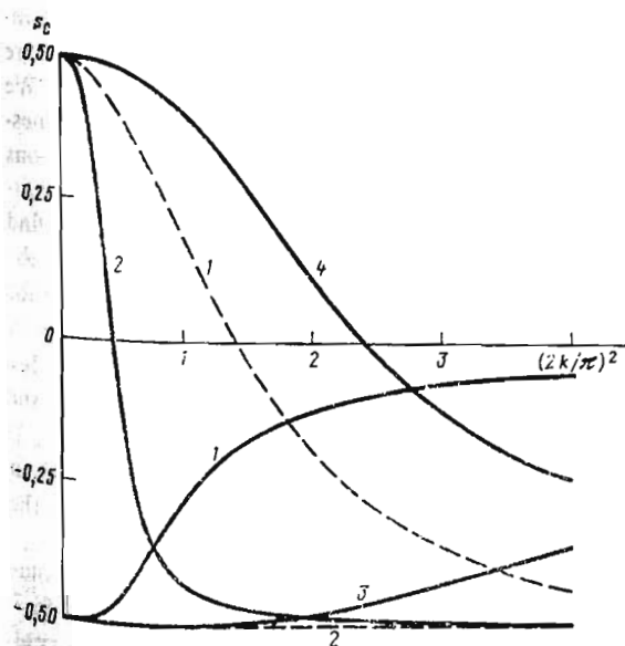
FIG. 4. Dependence of the average spin s_0 on k^2 for electrons photoexcited to the first size-quantized level. The notation is the same as in Fig. 3.
