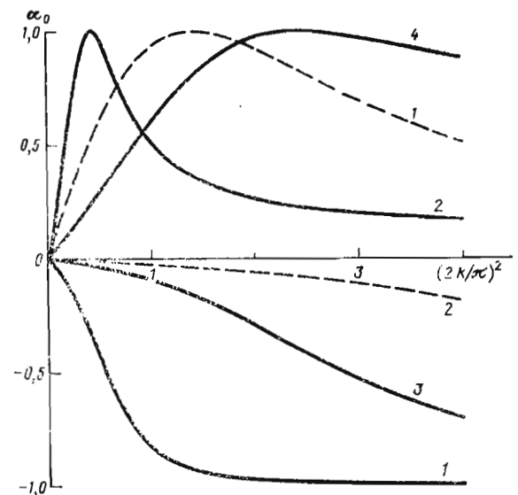
FIG. 3. Dependence of the alignment parameter \alpha_0 on k^2 for electrons photoexcited to the first size-quantized level. The half-width of the well is taken to be the unit of length. We use the spherical approximation with \nu = 0.18 . The solid curves are transitions from the heavy-hole subbands, the dashed are from the light-hole subbands. The numbers on the curves label the hole subbands.
