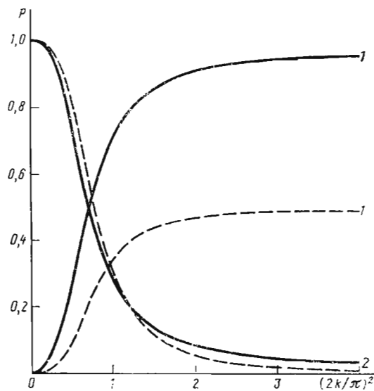
FIG. 7. Dependence of the linear ( P_l ) and circular ( P_c ) polarizations of the luminescence on k^2 for the process 1hh-1e-1hh . The dashed curves are the spherical approximation, v = 0.18 . The solid curves are the diagonal approximation with \gamma_1 = 6.79 , \gamma_2 = 1.924 , \gamma_3 = 2.681 (GaAs, Ref. 13). 1— P_l , P_{l\max} , 2— P_c .
