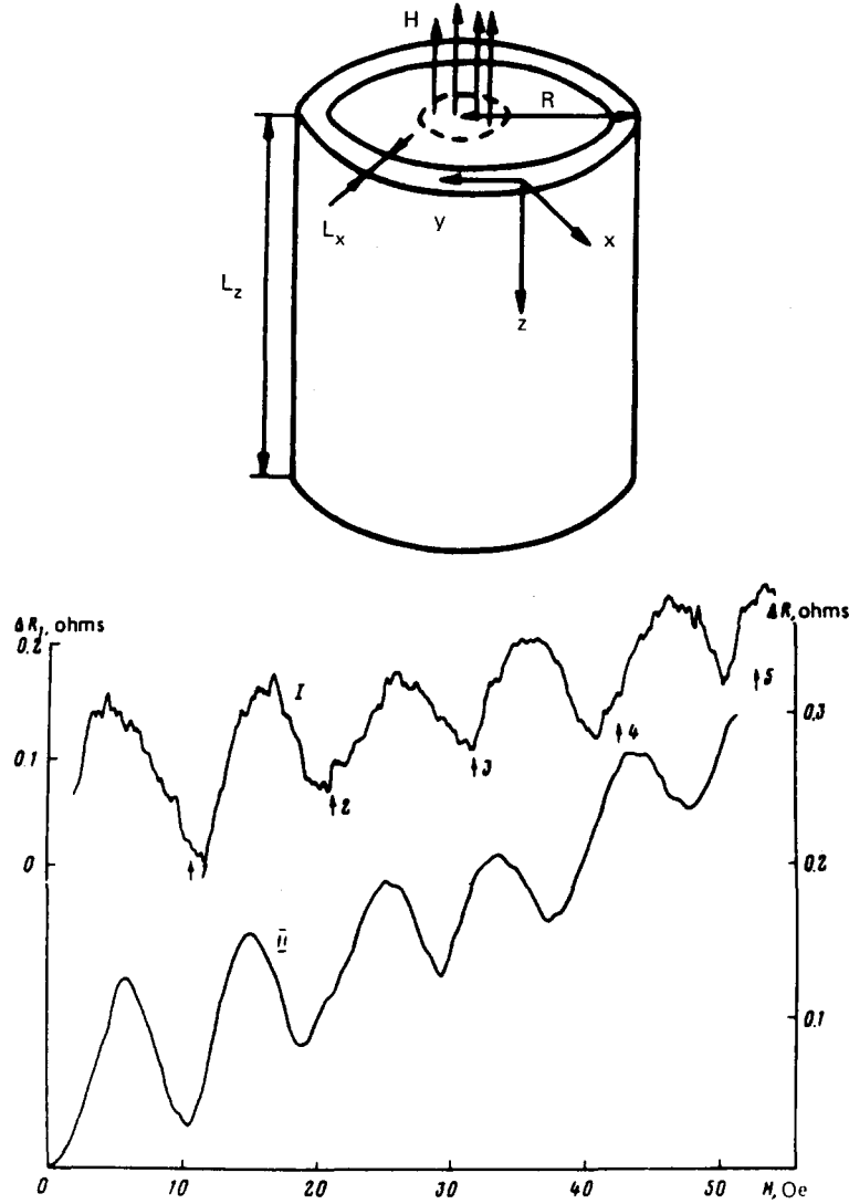
Fig. 2.7. Aranov-Bohm effect in a disordered hollow cylinder in a magnetic field parallel to the cylinder axis as suggested by Altshuler and Aronov [19], (a) the geometry, (b) the resistance oscillation as a function of the applied magnetic field measured by Sharvin and Sharvin [92] on a cylindrical Mg-film.
