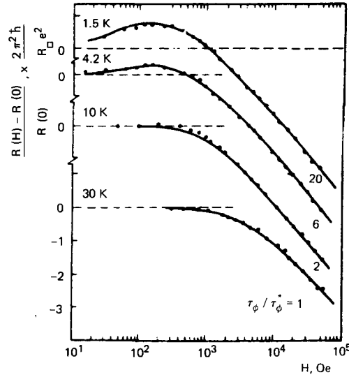
Fig. 5.2. The magneto-resistance of a thin Ag-film taken from Gershenson et al. [103]. The points are experimental results and the full curves theoretical ones.
