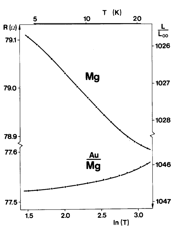
Fig. 5.7. The resistance (i.e. the normalized conductance L/L_{00} using the right scale) as function of \ln(T) for a Mg-film with a thickness of 84 Å. The same measurement after a superposition with 0.25 atola Au and another annealing at 40 K.
