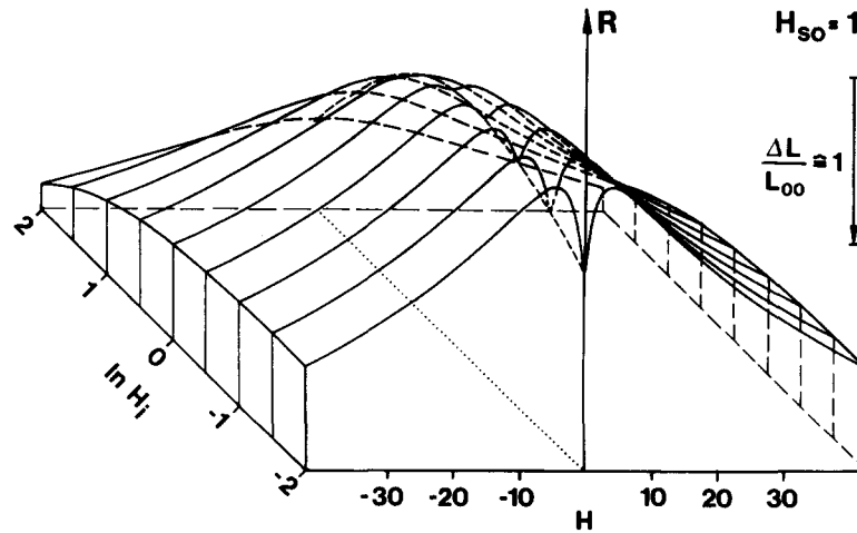
Fig. 4.3. The resistance (normalized conductance \Delta L/L_{00} ) as a function of the applied magnetic field H . H_{s0} is set equal to 1 and H_s = 0 . The third axis gives the parameter \ln(H_i) .
