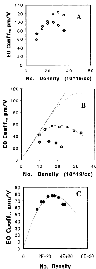
Fig. 2. Graphs of r_{33} as a function of chromophore number density are shown for several CLD- and FTC-type chromophores (Fig. 1). (A) Data for CLD-2 (circles) and CLD-3 (diamonds) show the effect of chromophore shape on maximum achievable r_{33} . The \mu\beta values are somewhat different for CLD-2 and CLD-3, making the initial slopes of the curves different. (B) Analogous data for FTC-1 (diamonds) and FTC-2 (circles) chromophores, again showing the influence of chromophore shape on achievable EO activity. Also shown are theoretical simulations assuming no intermolecular electrostatic interactions (solid straight line), full intermolecular interactions with chromophores treated as spheres (dashed line), and full intermolecular interactions with chromophores treated as ellipsoids (solid curving line). The ellipsoidal shape was defined by Spartan (WAVEFUNCTION, Inc., Irvine, California) calculations. (C) Experimental (solid circles) and theoretical (solid line) data compared for a variant of CLD-1, where the OTBDMS (tetra- n -butyldimethylsiloxane) protecting group has been replaced by a methoxy group. The theoretical curve was computed without adjustable parameters and explicitly incorporates nuclear repulsive interactions (as well as electronic interactions) treating chromophores as ellipsoids. The somewhat poorer agreement [relative to the FTC simulation of (B)] reflects neglect of higher order self-consistency (medium dielectric) effects in the calculations. Experimental data were taken at 1060 nm.
