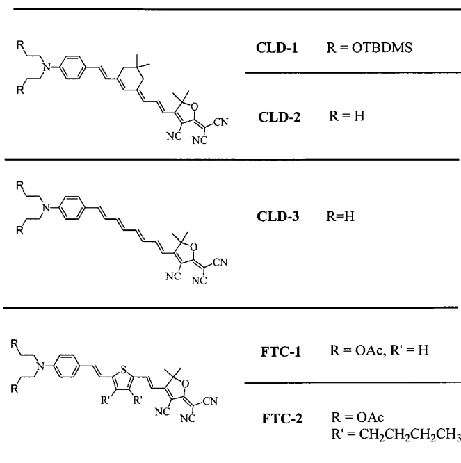
Fig. 1. Structures and abbreviated names of the chromophores discussed here. OTBDMS stands for the tetra- n -butyldimethylsiloxane protecting group; OAc stands for the acetate protecting group.
