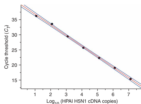
Figure 4 On-chip RT-PCR. The C_T values of seven separate experiments were plotted versus the log of the number of HPAI H5N1 cDNA copies. The solid black circles are C_T values; the solid red line is a linear regression fit ( R^2 = 0.999 ) of the C_T values; the solid blue lines denote the upper and lower 95% confidence limits. The PCR efficiency ( E ) was 93%, E = 10^{(-1/\text{slope})} - 1 . 1.2 - 1.2 \times 10^7 copies of HPAI H5N1 cDNA were used in 500 nl RT-PCR mixture.
