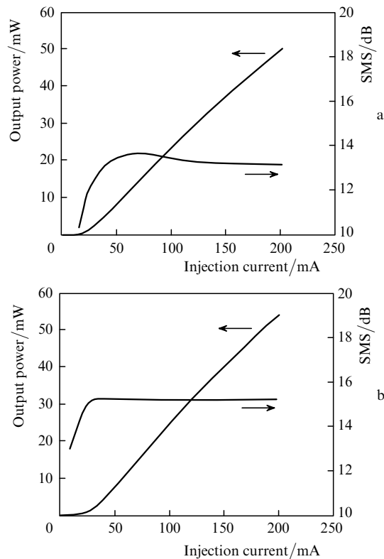
Figure 6. Output characteristics of the MOPA systems containing master oscillators (double-pass SLDs) with \Delta\lambda_{\text{FBG}} = 3.0 (a) and 0.5 nm (b).
