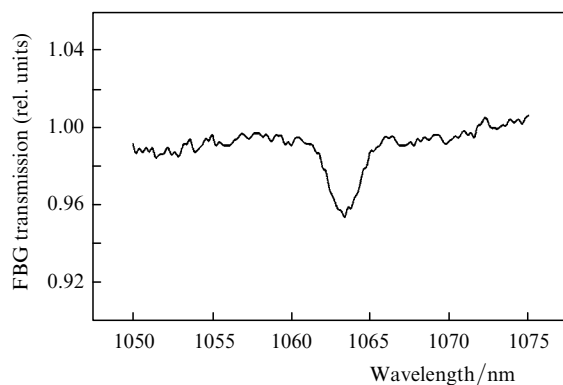
Figure 1. FBG transmission spectrum measured using a BS-1060-01 tunable laser.
