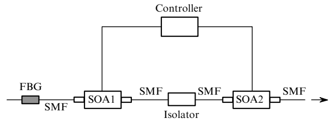
Figure 5. Schematic diagram of the MOPA.
