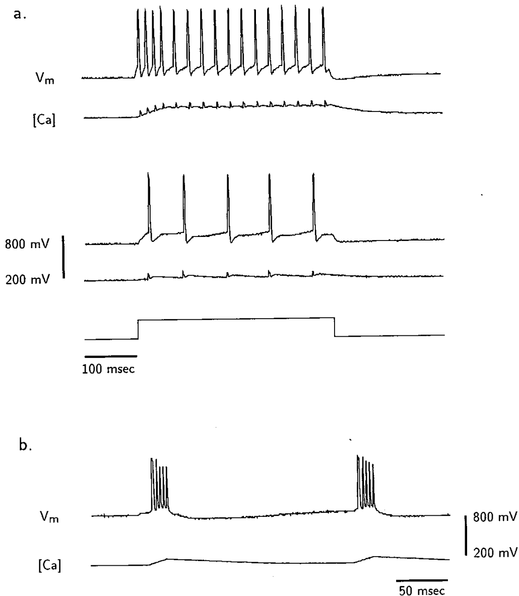
Figure 6 A silicon neuron that emulates the response of a cortical pyramidal neuron. (a) Response to two levels of intrasomatic current injection (time course shown below). The neuron is configured as a regular adapting pyramidal cell. Each pair of response traces consists of the somatic membrane potential, V_m (800 mV scale bar), and a voltage that is proportional to the intrasomatic free calcium concentration, [Ca] (200mV scale bar). Notice the adaptation of discharge and after-train hyperpolarization in the upper voltage trace. The voltage response of the silicon neuron is ten times larger than that of a real neuron (Douglas & Mahowald 1994a). (b) Response to sustained current injection of neuron configured as a bursting pyramidal cell.
