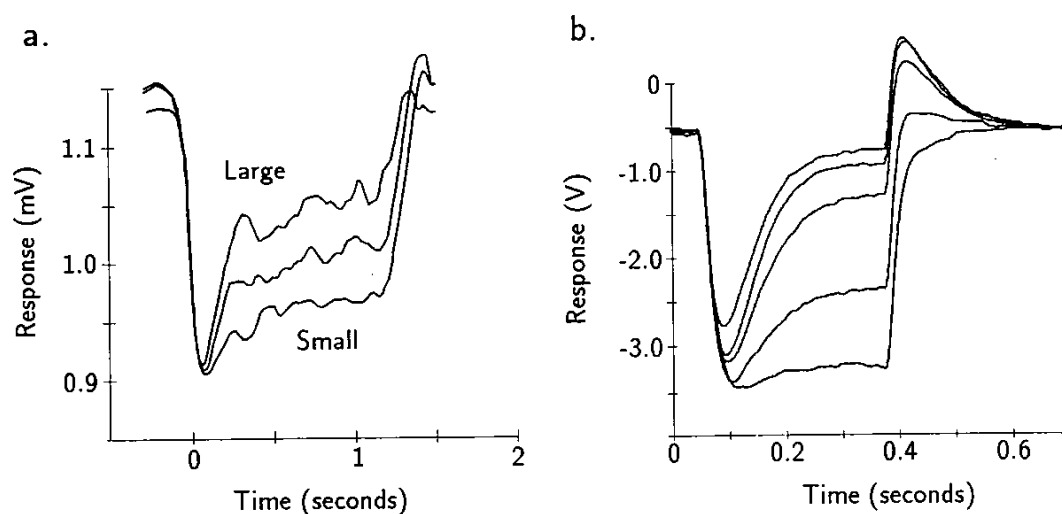
Figure 3 Comparison of the response of bipolar cells in a vertebrate and a silicon retina to a flashing light stimulus of varying spatial extent. (a) Response of a bipolar cell in the mud puppy, Necturus maculosus (data from Werblin 1974). (b) Output of a pixel in the silicon retina. Test flashes of the same intensity but of different diameters are centered on the receptive field of the unit. Larger flashes increase the excitation of the surround. The surround response takes time to build up to the capacitance of the resistive network. Because the surround level is subtracted from the center response, the output shows a decrease for long times. This decrease is larger for larger flashes. The overshoot at stimulus offset decays as the surround returns to its resting level. The peak response diminishes as the test flash becomes larger spatially. The larger test flash charges the network to a higher value. The charging of the network works against the finite response time of the receptor to produce the observed decrease in peak response at the bipolar cell level.
