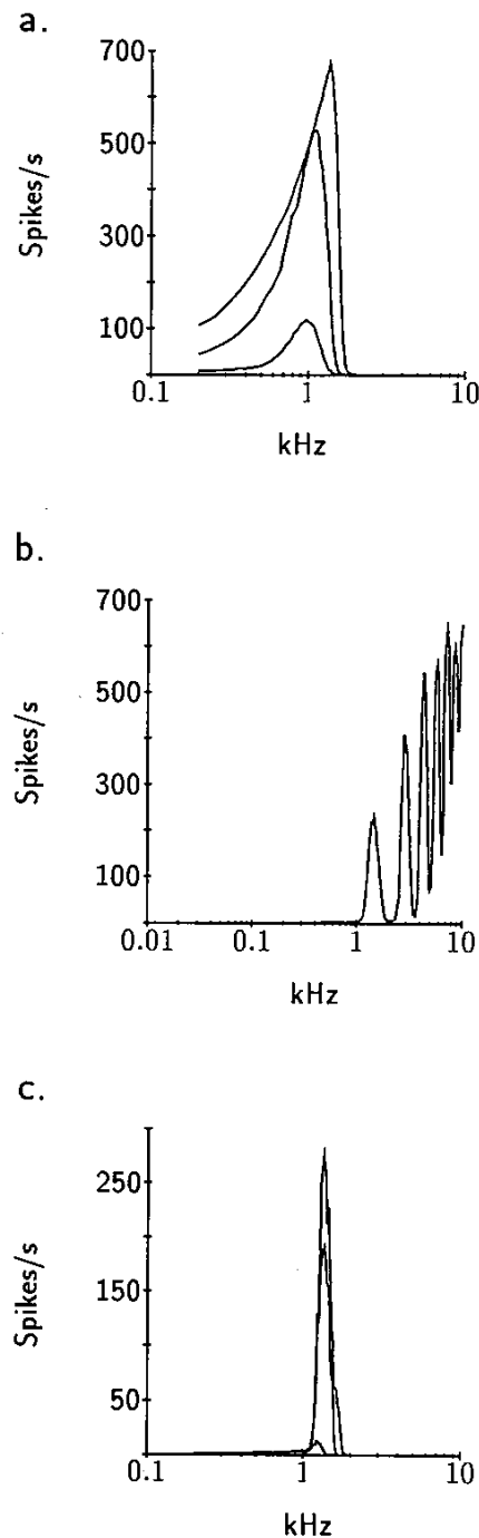
Figure 4 Response of a silicon auditory processor that emulates a cochlea, auditory neurons, and proposed postsynaptic neurons that act as correlators. (a) Average discharge rate of the auditory neurons in response to sinusoidal stimuli (2, 5, and 20 mV peak amplitude, bottom to top) applied to the cochlea. Notice that the bandwidth of the response is sensitive to input amplitude. (b) Output from a correlator postsynaptic to the auditory fibers shown in a, with cochlea filtering disabled. The correlator responds at its optimal frequency (about 1.5 kHz) with narrow bandwidth, but it also responds at higher harmonics. (c) Output of the correlator to the stimuli described in a, with cochlea filtering enabled. The response is logarithmic over the stimulus range 2–20 mV. There are no harmonics. The bandwidth is insensitive to stimulus amplitude. The auditory processor responds to frequencies over a range of approximately 0.3–3 kHz (data not shown). Modified from Lazzaro 1991.
