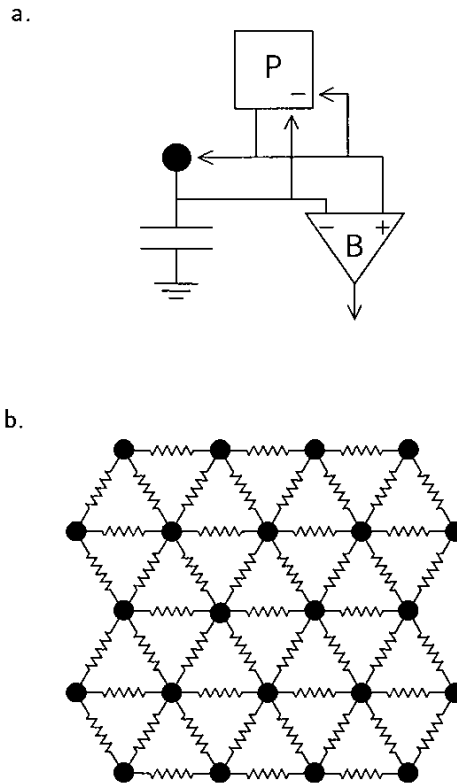
Figure 2 The silicon retina is a two-dimensional hexagonal array of pixels on a chip. The retina transduces a light image focussed directly on its surface, processing the stimulus by principles found in the outer plexiform layer of the vertebrate retina. Various versions of silicon retinæ contain from 2304 (Mahowald & Mead 1989) to 8250 pixels (Boahen & Andreou 1992) on a 6.8 mm × 6.9 mm square of silicon using a 2- \mu m fabrication process. (a) A pixel from the silicon retina produced by Mahowald (1991) contains an analogue of a photoreceptor, P, a bipolar cell, B, and a node of the horizontal cell network ( filled circle ). (b) A hexagonal resistive network emulates the horizontal cells of the retina. The horizontal cells extend parallel to the surface of the retina and are resistively coupled to each other by gap junctions. The values of these resistors is controlled by applying an analogue voltage to the chip, so the degree of connectivity between horizontal cells can be varied after the chip is fabricated. In addition to the retinal array, the retina chips also have instrument circuits that monitor the outputs of the pixels. The pixels can be monitored individually or scanned out sequentially to a video monitor.
