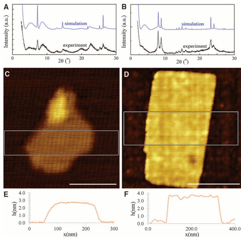
Fig. 2. Powder XRD pattern from MWW nanosheets (A) and MFI nanosheets (B). a.u., arbitrary units. The bottom traces show experimental XRD patterns (Cu K \alpha source, wavelength = 1.5418 Å) of the powder obtained by calcination of the nanosheet-polystyrene nanocomposite at 540°C. The top traces are the simulated XRD patterns (powder pattern theorem, implemented with UDSKIP) of the proposed structure of the nanosheets. AFM (tapping mode) topographical images of MWW and MFI nanosheets are shown in (C) and (D), respectively. The average step-height ( h ) data of the area highlighted in (C) and (D) are plotted in (E) (MWW nanosheet) and (F) (MFI nanosheet). The height data are calibrated using steps formed on freshly cleaved mica. Scale bars in (C) and (D), 200 nm.
