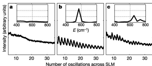
Fig. 17 Liquid phase single-pulse CARS spectroscopy of three organic substances. 264 As laser pulse trains are generated by different sinusoidal spectral phase patterns, the CARS signal is plotted as a function of the corresponding periods across the spatial light modulator (SLM). The derived Raman spectra are shown as inset. The three data sets correspond to (a) methanol (no resonance in the accessible frequency range), (b) \text{CH}_2\text{Br}_2 (one resonance), and (c) (\text{CH}_2\text{Cl})_2 (two resonances), where the CARS signal shows a clear beating between the two accessible Raman modes. Reprinted with permission from the authors and from Macmillan Publishers Ltd: N. Dudovich, D. Oron and Y. Silberberg, Nature , 2002, 418 , 512, Copyright 2002.
