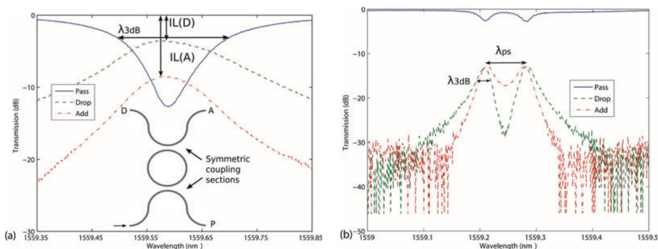
Figure 12 (online color at: www.lpr-journal.org ) Spectra at the pass, drop and add port for a microring resonator with radius 5 μm and a gap of (a) 200 nm and (b) 400 nm using TE-polarized light and with cross section depicted in Fig. 7(a). In (b) the Q-factor becomes high enough to see resonance splitting. Moreover the output power level at the add port becomes comparable with the output power level at the drop port.
