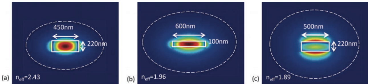
Figure 7 (online color at: www.lpr-journal.org ) Illustration of the mode spreading in three SOI waveguide cross sections (core n_{Si} = 3.48 , cladding n_{SiO_2} = 1.54 ). (a) standard waveguide for TE polarized light (b) reduced interaction with vertical sidewalls and lower confinement, waveguide cross section used in [38] for the TE polarization (c) using TM-polarized light, no discontinuity at vertical sidewalls and lower confinement, waveguide cross sections used in [31].
