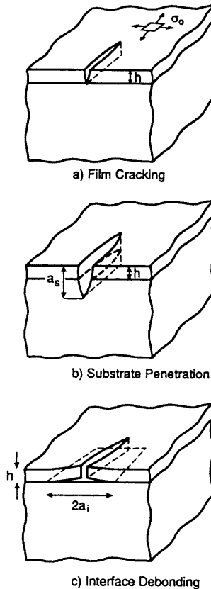
Fig. 1. (a) A channeling crack within a thin film. (b) A channeling crack penetrating into the substrate. (c) A channeling crack with interface debonding.
