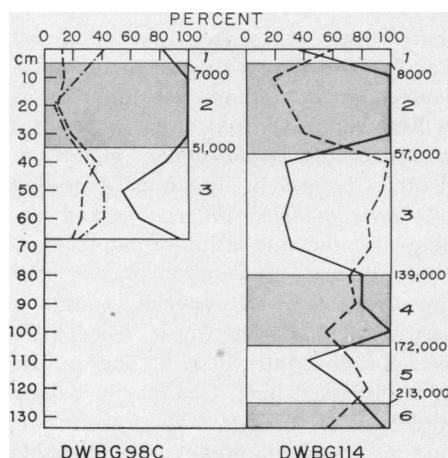
Fig. 2. Proportional contributions of the end members DWBG 61 (solid line), R69G (dash-dotted line), and R30G (dashed line). The odd-numbered intervals represent present-day oceanographic conditions; shaded even-numbered intervals represent oceanographic conditions in which there was displacement of high-latitude fauna toward the equator. The smaller numbers to the right of the cores are the ages of the boundaries between the intervals.
