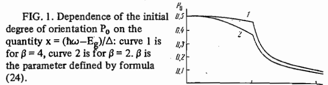
FIG. 1. Dependence of the initial degree of orientation P_0 on the quantity x = (\hbar\omega - E_g)/\Delta : curve 1 is for \beta = 4 , curve 2 is for \beta = 2 . \beta is the parameter defined by formula (24).
