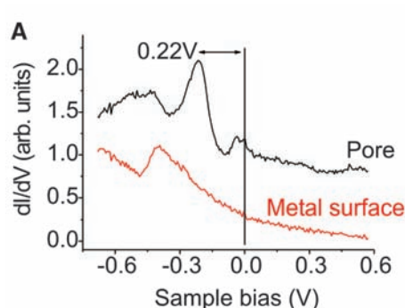
Fig. 2. Study of the electronic confinement of the surface state within the pores of the network, corresponding to an array of 0D quantum dots. (A) STS spectra obtained at 5 K on the clean Cu surface (red) and inside a pore of the dehydro-DPDI network (black). The latter spectrum exhibits a maximum at -0.22 V, which is attributed to a confined surface state (lock-in: V_{rms} = 6 mV, f = 513 Hz, initial tip parameters: -0.8 V/80 pA). (B) STM image of the porous network (13.6 nm by 13.6 nm, -0.20 V, 70 pA) and (C) simultaneously recorded dI/dV map at 5 K (lock-in: V_{rms} = 8 mV, f = 513 Hz). A confined electronic state is observed inside the molecular pores. The black
