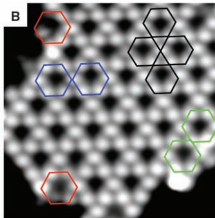
Fig. 1. Interaction of the dehydro-DPDI network with the surface state of the underlying substrate. The formation of this porous network is based on a thermally induced dehydrogenation of DPDI on Cu(111). (A) Molecular structure of DPDI and its dehydrogenated form. (B) STM image for submonolayer coverage of DPDI deposited on Cu(111) after thermal annealing at 500 K. Dehydro-DPDI acts as both hydrogen-bond donor and acceptor to produce a very stable self-assembled porous network (image size: 29 nm by 29 nm, -0.1 V, 50 pA) (21). The network periodicity is 2.55 nm with a pore diameter of \sim 1.6 nm. Standing wave patterns in the Cu surface state arise from the scattering of the delocalized electronic states at the border of the adsorbate adlayer. This can be observed at low tunneling bias (4–6).
