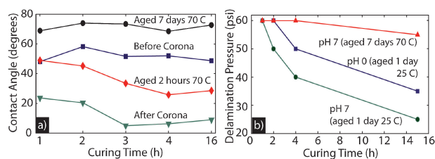
Fig. 7 (a) Water contact angles before and after corona treatment of cured silane layers. Hydrophobic recovery is slower for samples with prolonged curing times. (b) Delamination pressure of blisters after a 2 hour water bake at 70 °C. Samples are bonded with corona treatment to PDMS after specified silane curing times. Delamination pressure decreases for samples bonded after longer curing times, but improves after aging bonded structures for 1 week at 70 °C. Similar behaviors of contact angle and delamination pressure suggest that interface hydrophobicity plays a major role in hydrolytic resistance.
