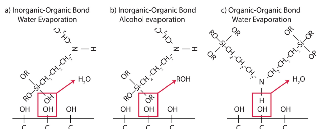
Fig. 2 Different methods of bond formation between organofunctional silanes and organic substrates. Inorganic–organic bond formation can occur through water (a) or alcohol (b) evaporation, generating Si–O–C bonds. Organic–organic bond formation can also occur through water evaporation (c).
