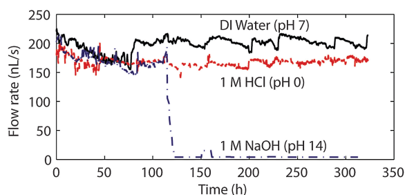
Fig. 10 Plot of the flow rate versus time for three different peristaltic pumps flowing different pH solutions at 18 psi. Pumping rate is 1 cycle every 500 ms. Marginal decrease in flow rate over the course of the experiment demonstrates long term bond reliability.
