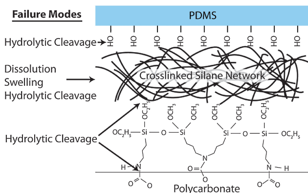
Fig. 3 Different bond failure mechanisms for silane bonding between organic substrates and PDMS. The PDMS–silane interface, the PC–silane interface, and the silane network are all vulnerable to hydrolysis.
