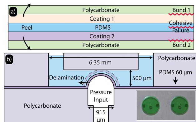
Fig. 5 (a) Schematic of the bond stack used for peel tests. PC layers are bonded to a PDMS membrane using silane coatings on either side. (b) Schematic of the aqueous blister test structure used to test hydrolytic bond failure. Suspended PDMS membranes were 60 \mu\text{m} thick and 915 \mu\text{m} in diameter. A picture of a fabricated blister test structure with the wells loaded with green dye is shown in the inset.
