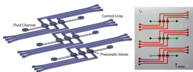
Fig. 9 Schematic and picture of the test device fabricated in PC utilizing a 60 \mu\text{m} PDMS membrane to provide pressure based actuation valves. Control lines are 500 \mu\text{m} wide and 250 \mu\text{m} high. The fluid channel is 125 to 150 \mu\text{m} deep with a radius of curvature of 400 \mu\text{m} with a 1.6 mm valve length. Variation in depth results from machining inaccuracies.
