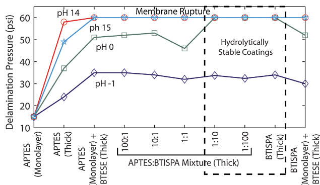
Fig. 8 Plot of the delamination pressure versus primer type at pH extremes. Dotted area shows coatings that were stable from pH 0 to pH 15. Optimal hydrolytic stability occurs when coatings contain a majority of BTISPA, with failure only occurring at pH -1.
