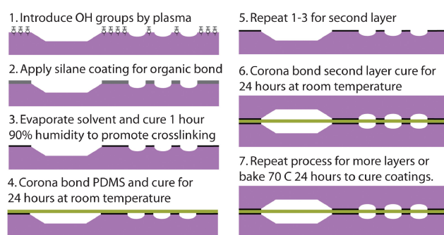
Fig. 4 Fabrication process for bonding PC to PDMS using silane coatings. Curing and annealing steps are intentionally prolonged to ensure bond formation and hydrophobic recovery.
